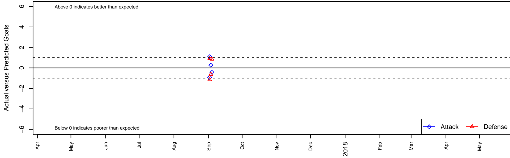
CCB Metro B05 Dots are actual minus expected GF (blue circles) and GA (red triangles). Blue line is smoothed change in attack strength. Red is smoothed change in defense strength.
